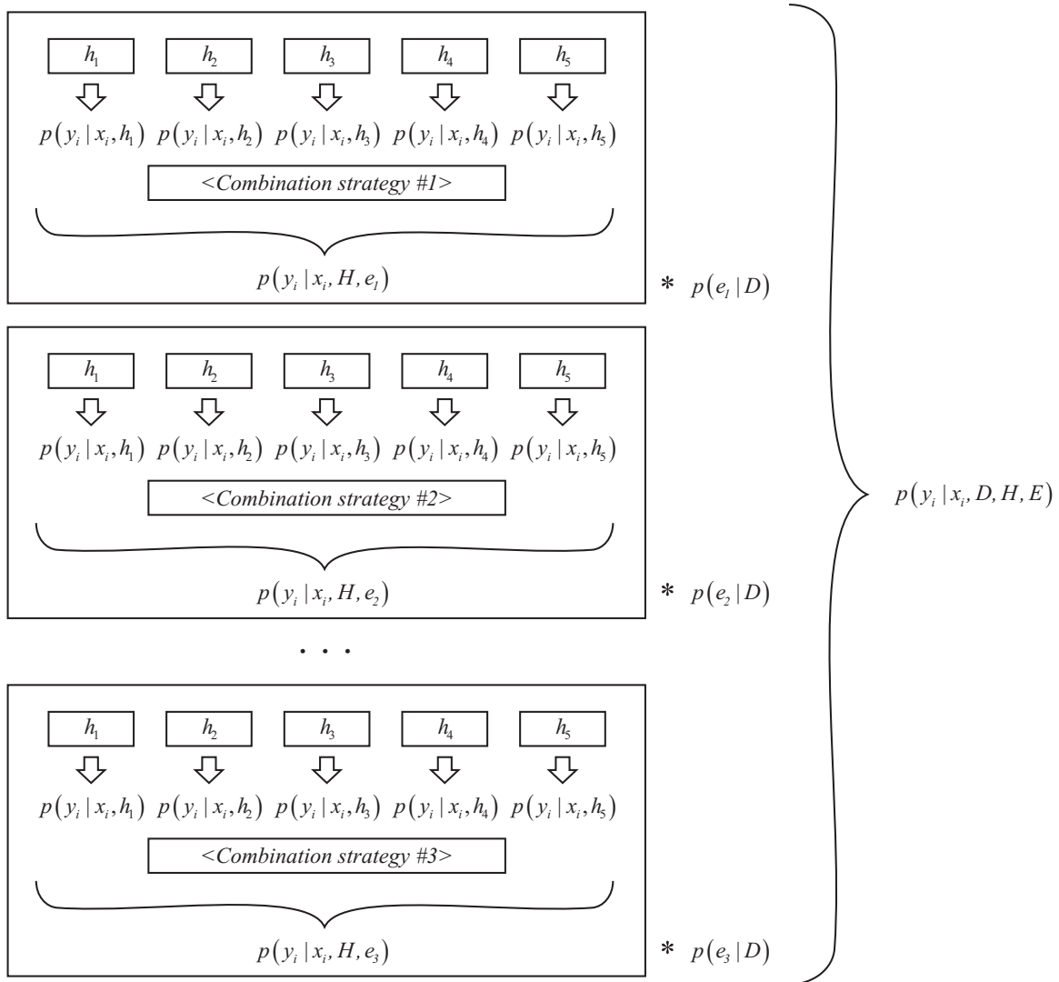
Figure 8.2: Bayesian Model Combination. In this case, p(y_i|x_i, D, H, E) will be predominantly determined by p(e_{mostLikely}|D) . The model is now heavily weighting the most probable combination of hypotheses instead of the most probable single hypothesis.
